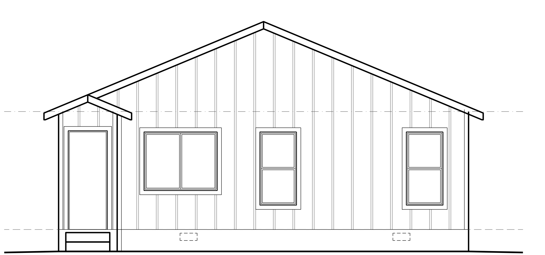
D LEFT ELEVATION A2.1 1/4" = 1'-0"
