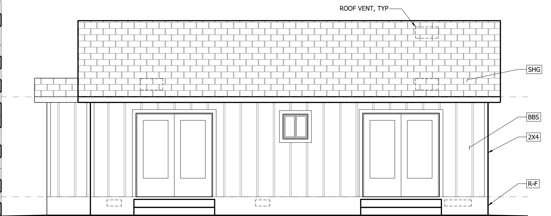
A FRONT ELEVATION A2.1 1/4" = 1'-0"
