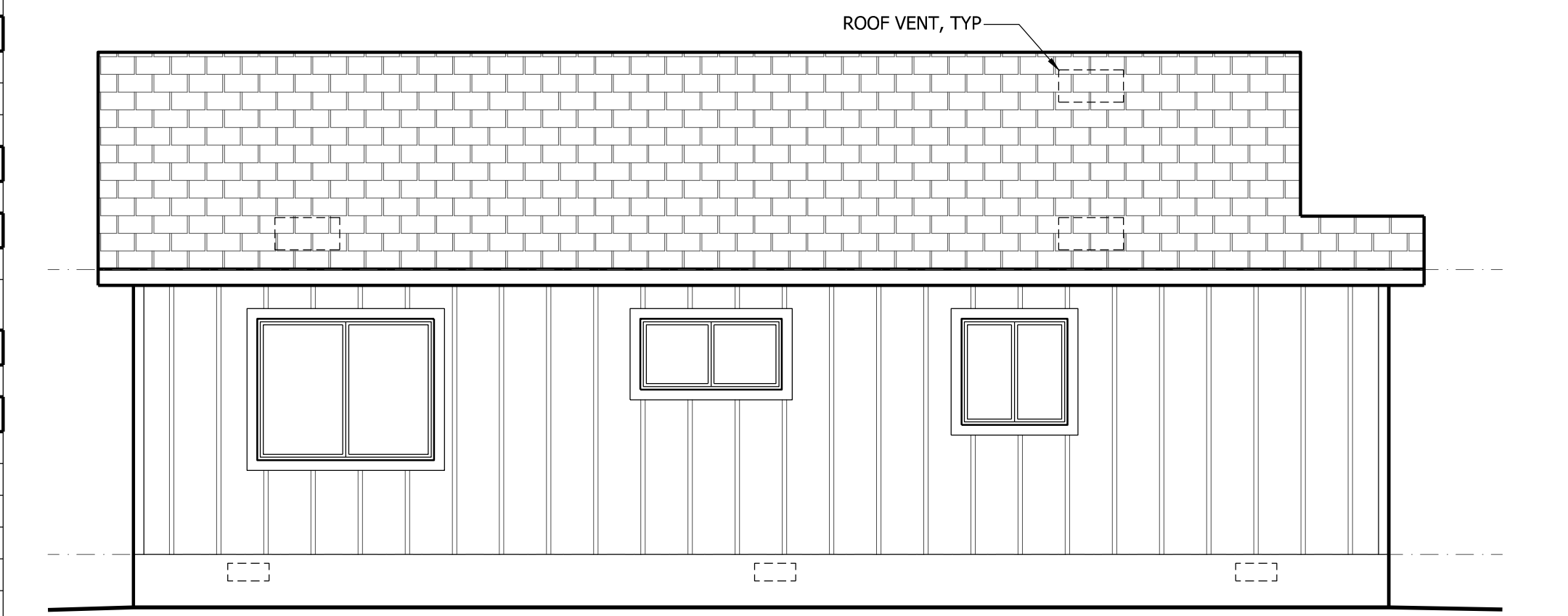
C REAR ELEVATION A2.1 1/4" = 1'-0"
