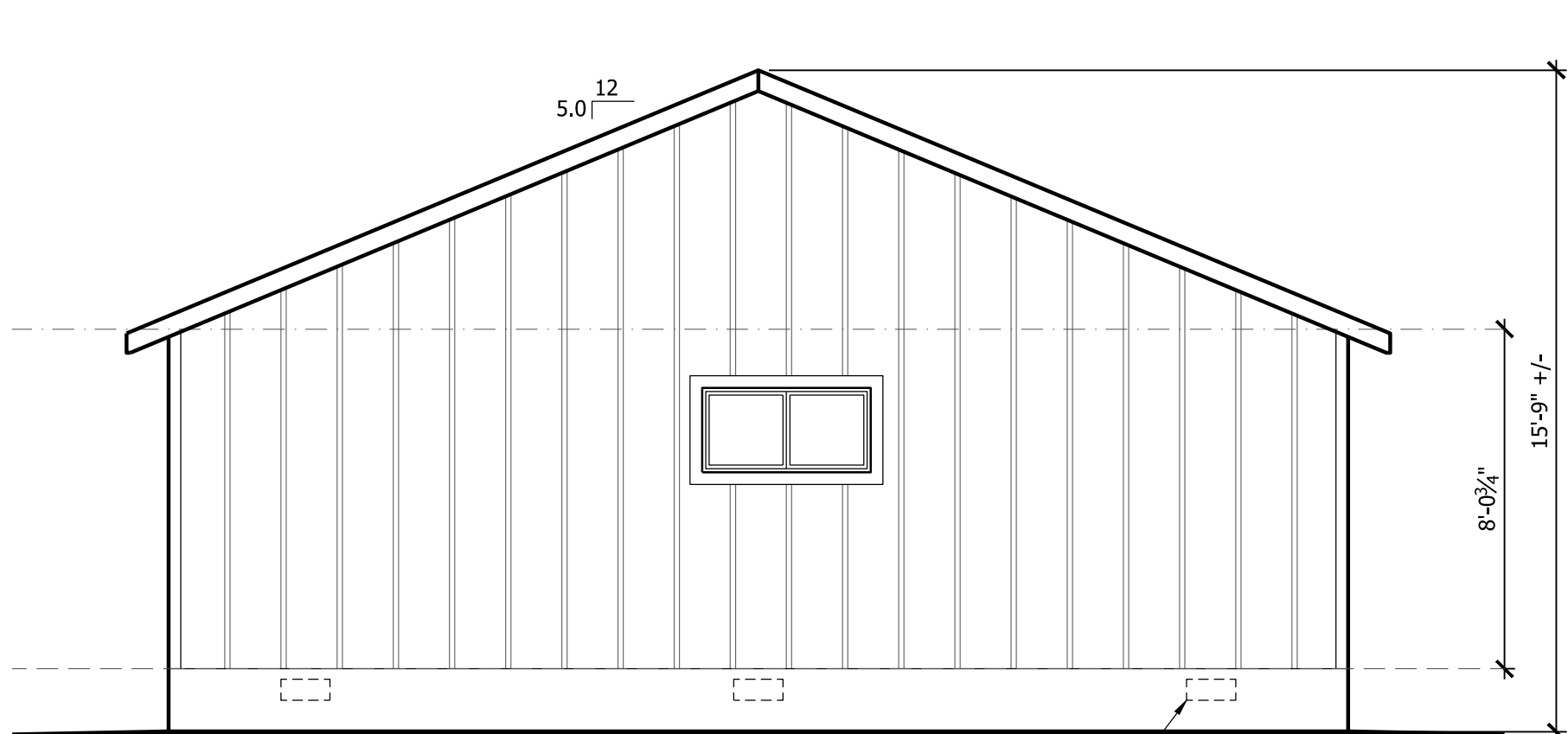
B RIGHT ELEVATION A2.1 1/4" = 1'-0"
