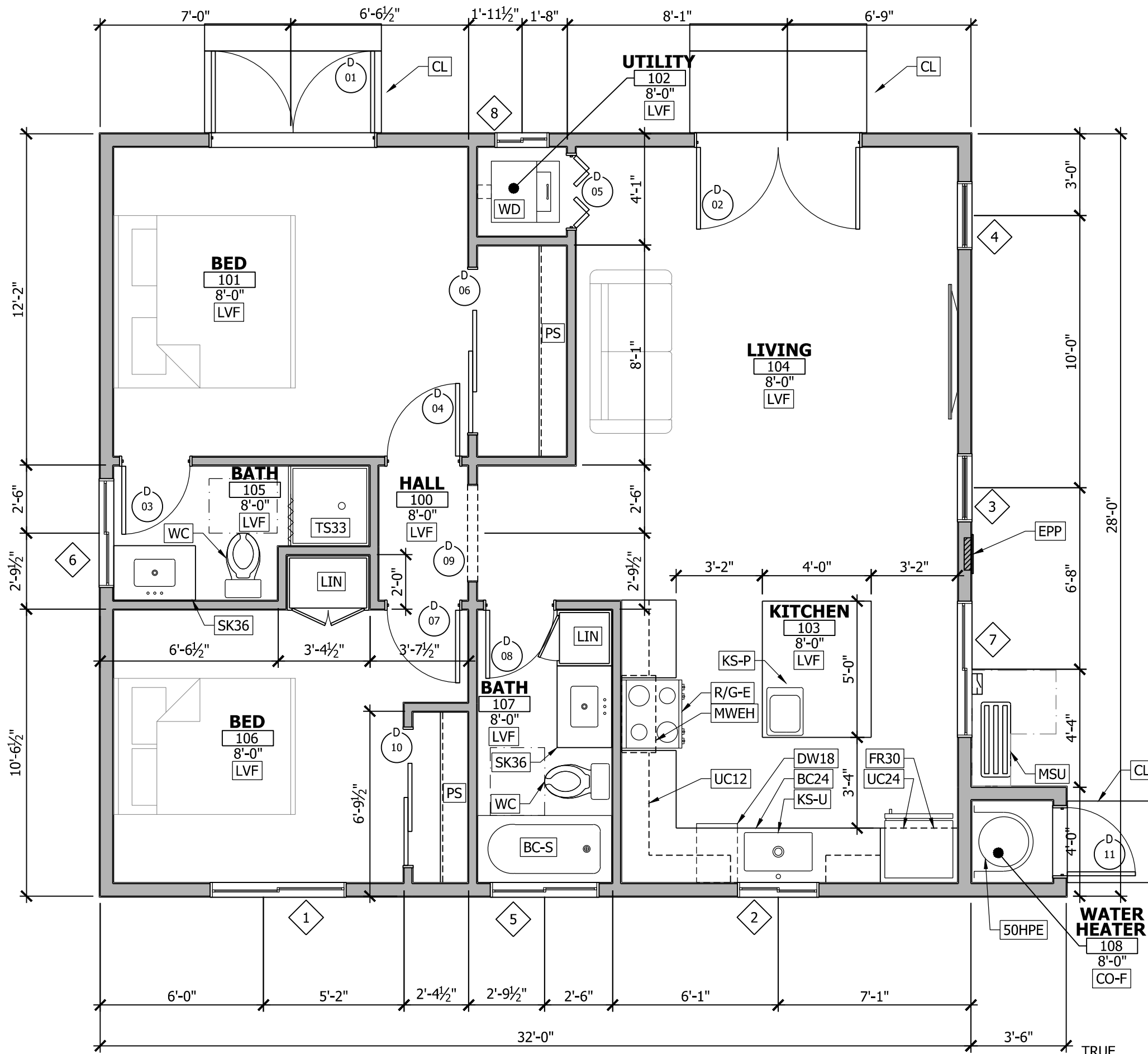
1 FLOOR PLAN A2.1 1/4" = 1'-0"
